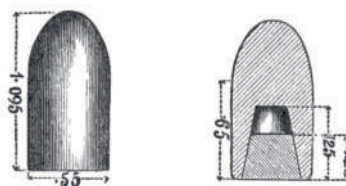
Fig. 1.—BULLET USED IN ENFIELD RIFLE.
